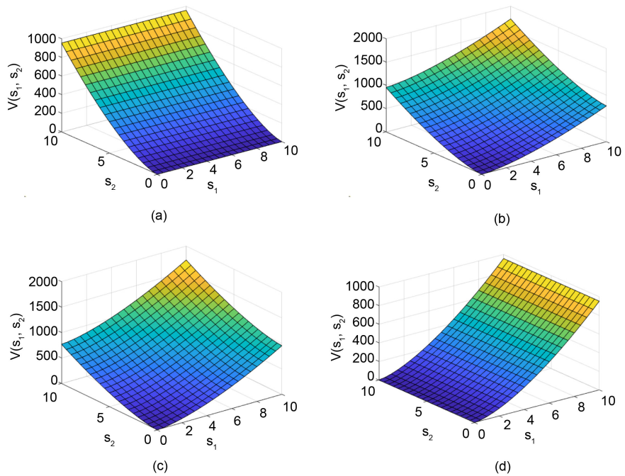
Figure 1. Illustration of how the total investment value function \tilde{V}(\bar{S}^*(t)) increases for various values of \alpha_i, i=1,2 . (a) For S_1(t) : \alpha_1=0 and for S_2(t) : \alpha_2=7 ; (b) For S_1(t) : \alpha_1=4 and for S_2(t) : \alpha_2=7 ; (c) For S_1(t) : \alpha_1=7 and for S_2(t) : \alpha_2=4 ; (d) For S_1(t) : \alpha_1=7 and for S_2(t) : \alpha_2=0 .
