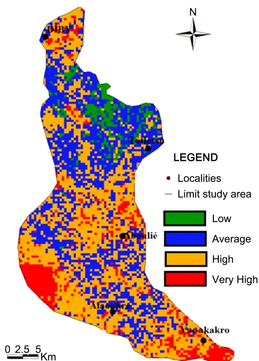
Figure 3. Map of vulnerability to pollution.
