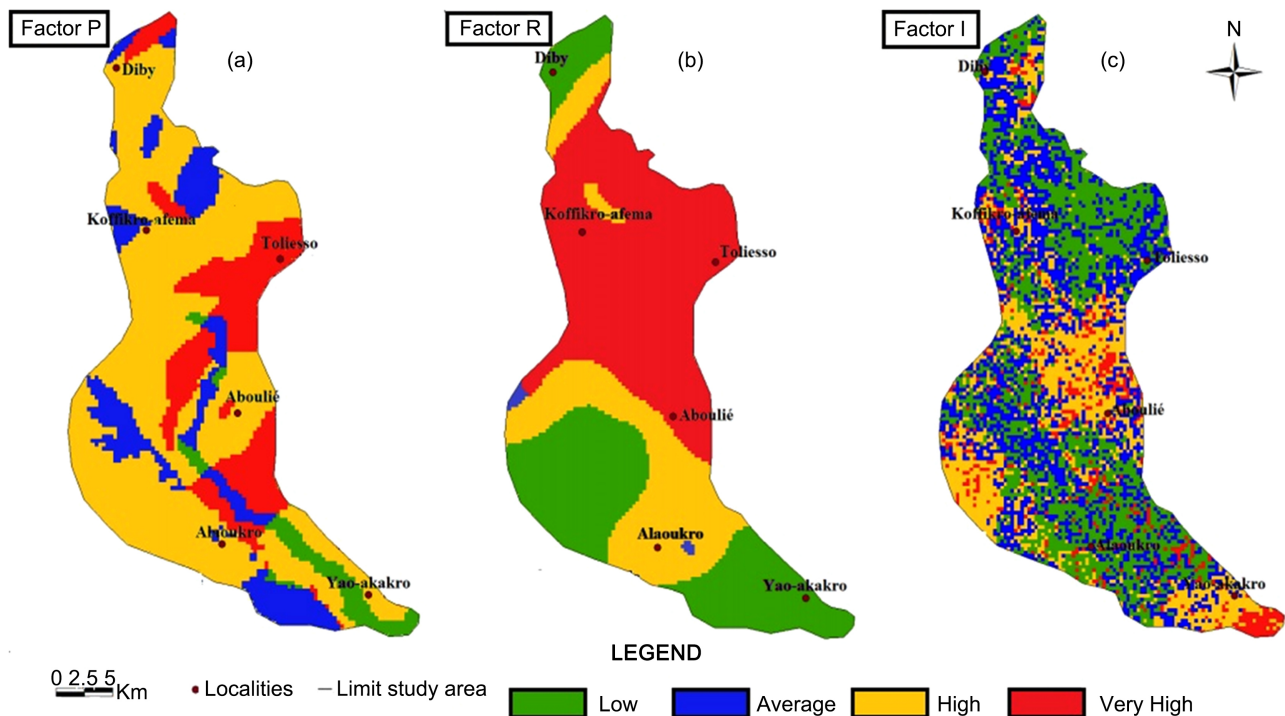
Figure 2. Maps of different factors: (a) Factor P (Protection); (b) Factor R (Reservoir); (c) Factor I (Infiltration).
