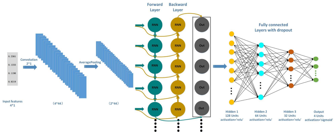
Figure 1. An illustration to show a dense neural network with 3 fully connected layers. Adapted from [11] with permission.
