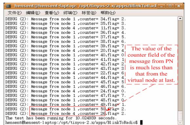
Figure 14. The debugging information for BlinkToRadio in H-TOSSIM.
