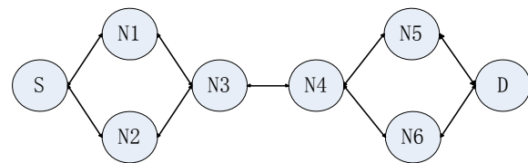
Figure 3. Non-disjoint multi-path.
