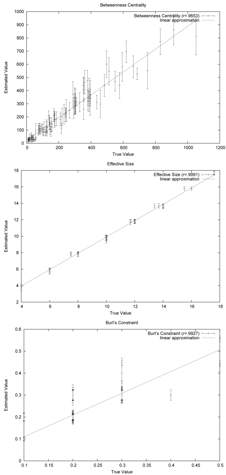
Figure 2. ECSTC on a 100 node network.
