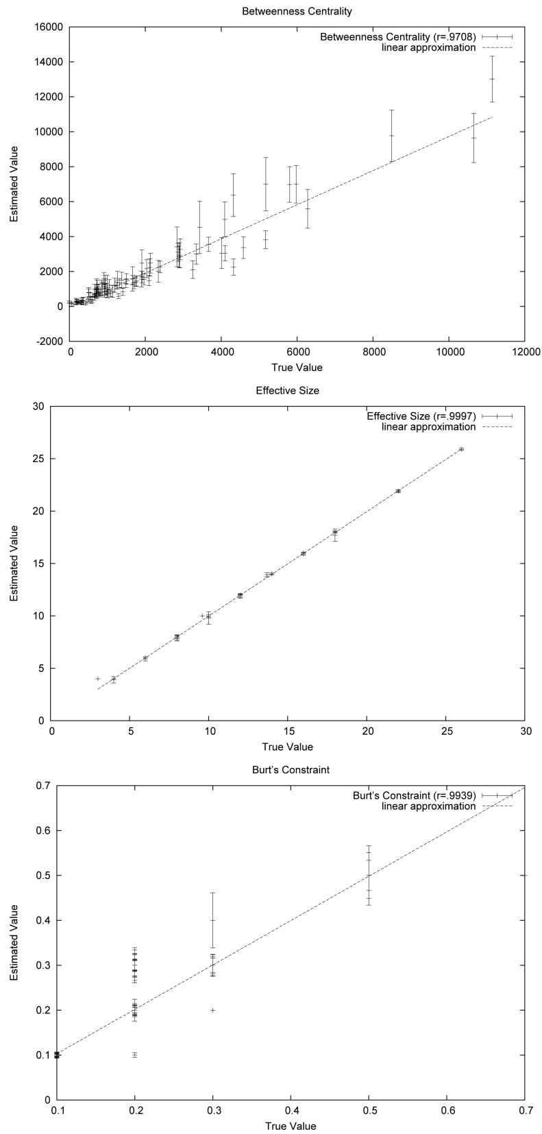
Figure 3. ECSTC on a 500 node network.
