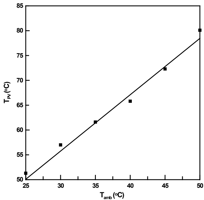
Figure 6. Variation of cell temperature against ambient temperature.
