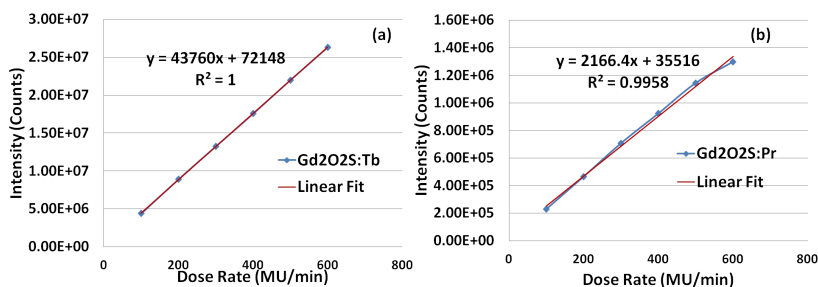
Figure 2. Intensity response at different dose rate for different Sensor materials (a) \text{Gd}_2\text{O}_2\text{S: Tb} . (b) \text{Gd}_2\text{O}_2\text{S:Pr} .
