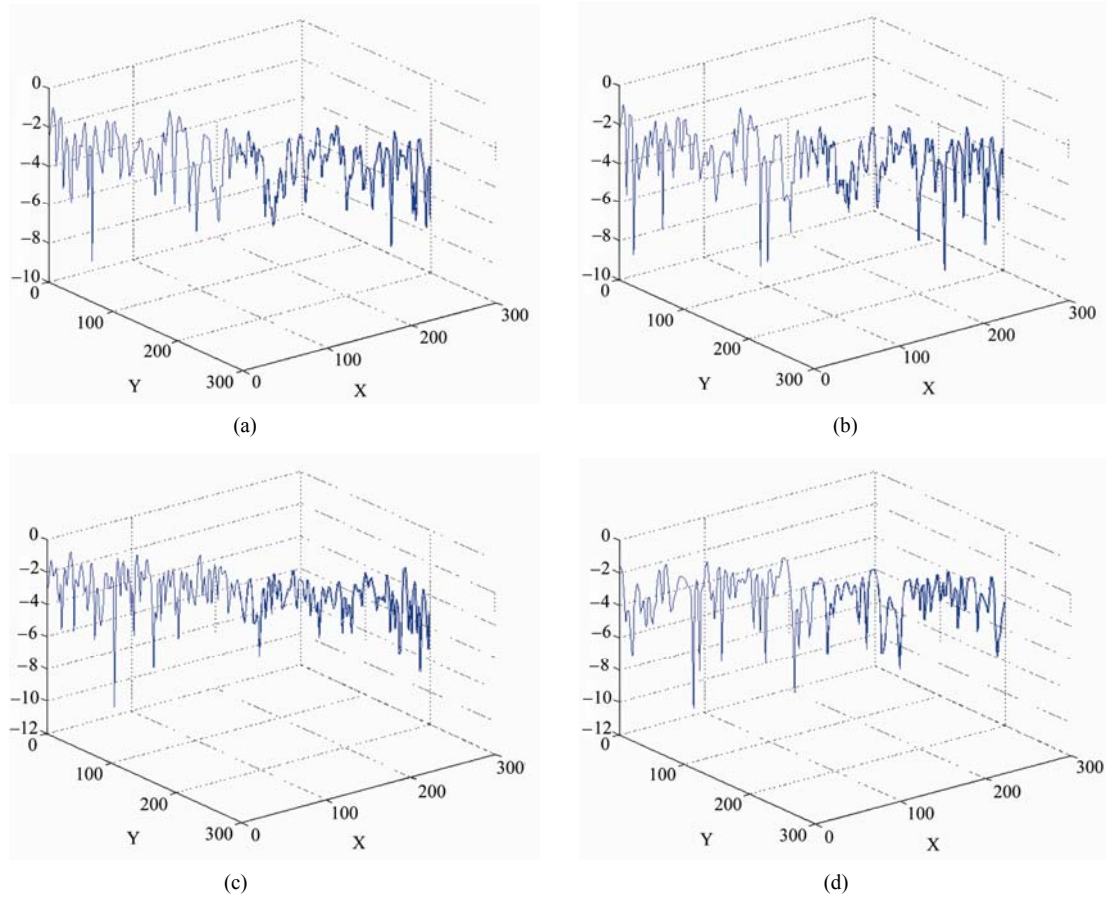
Figure 5. (a) The profile shape of the numerical speckle image obtained using the linearly distributed aperture; (b) The profile shape of the numerical speckle image obtained using the quadratic aperture; (c) The profile shape of the numerical speckle image obtained in case of \rho^{10} distributed aperture; (d) The profile shape of the numerical speckle image obtained in case of uniform circular aperture.
