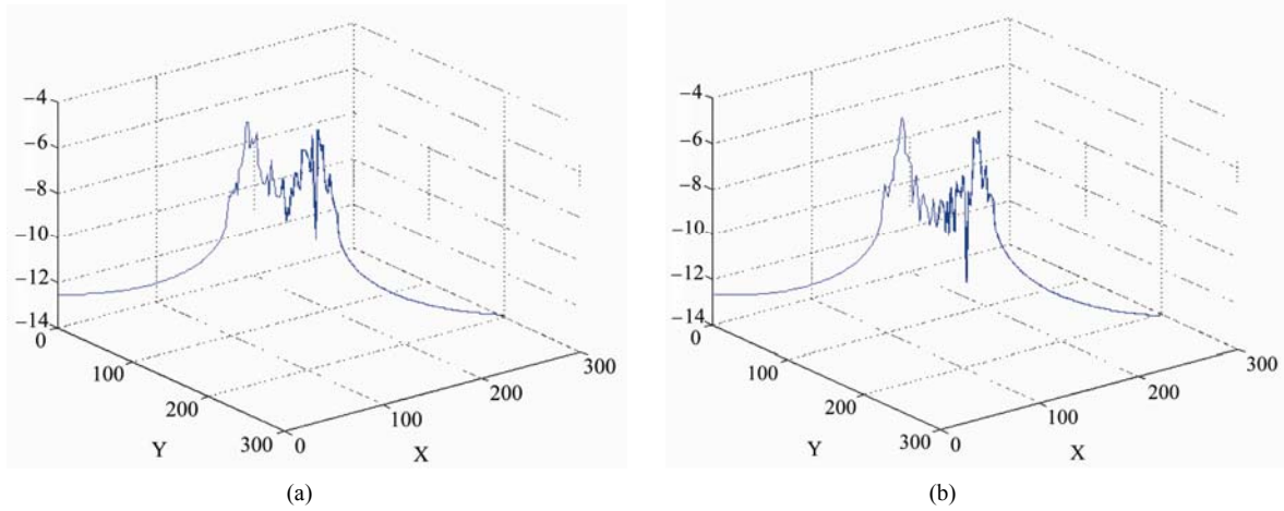
Figure 7. (a) Profile shape of the reconstructed quadratic aperture; (b) Profile shape of the reconstructed \rho^{10} aperture.
