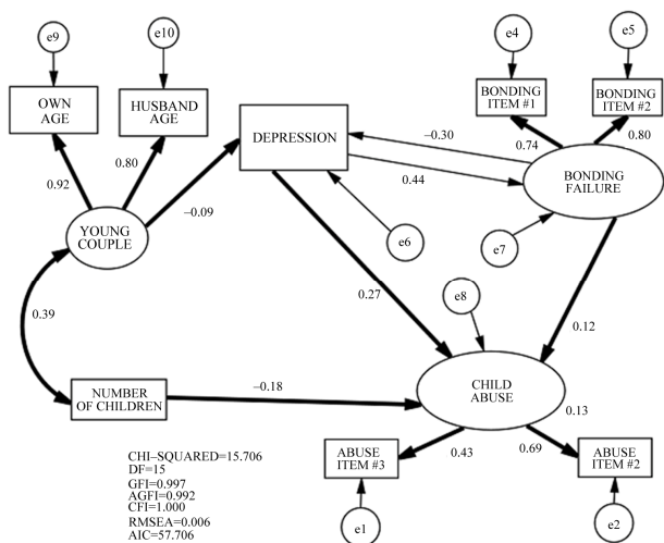
Figure 2. Final SEM model of the association between Bonding Failure, Depression, and Child Abuse. (Significant paths and covariances are in bold.)
