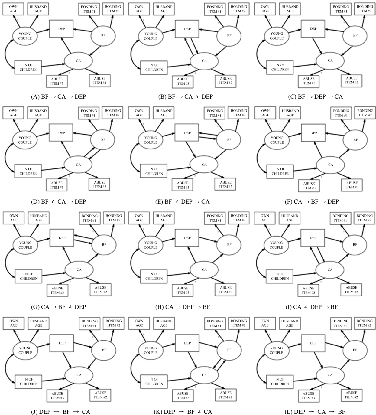
Figure 1. Multiple SEM models of the associations between Bonding Failure (BF), Depression (DEP), and Child Abuse (CA).
