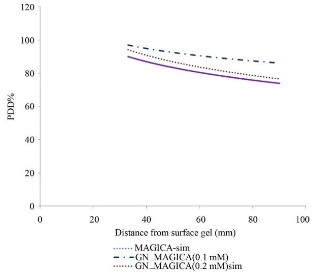
Figure 7. Comparison between MAGICA and GN_MAGICA percentage depth dose in simulation.
