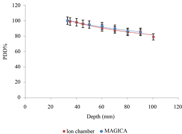
Figure 5. Percentage Depth Dose (PDD (%)) of curve MAGICA gel and ion chamber measured in water phantom.
