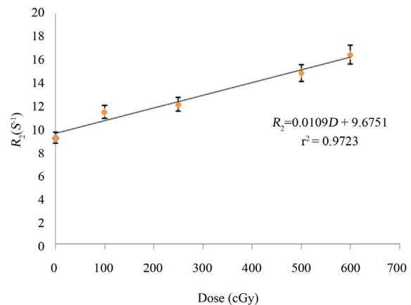
Figure 4. MAGICA polymer gel dosimeter R_2 response on absorbed dose in range of 0 - 600 cGy.
