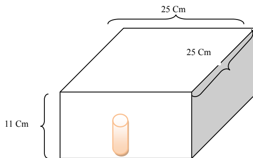
Figure 2. Geometry of simulated phantom.
