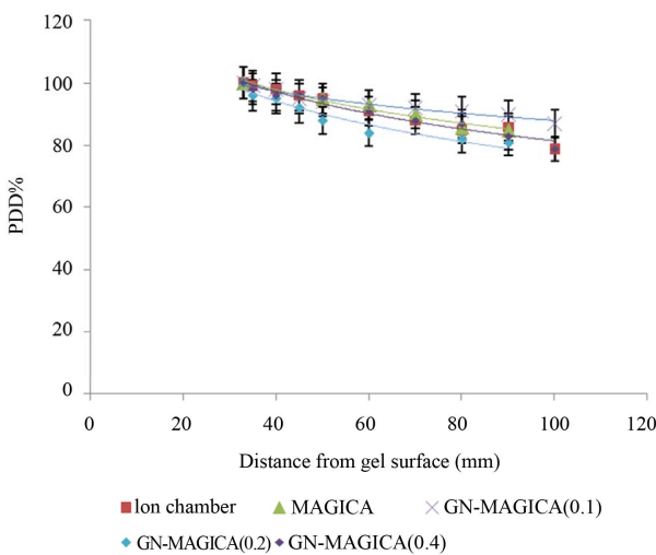
Figure 6. Comparison of three GNPs concentration with MAGICA depth dose curve.
