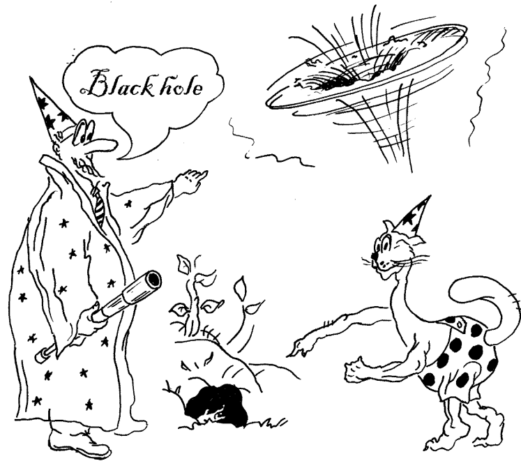
Figure 1. Black hole.
