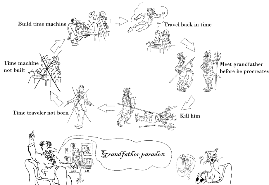
Figure 3. Grandfather paradox.
