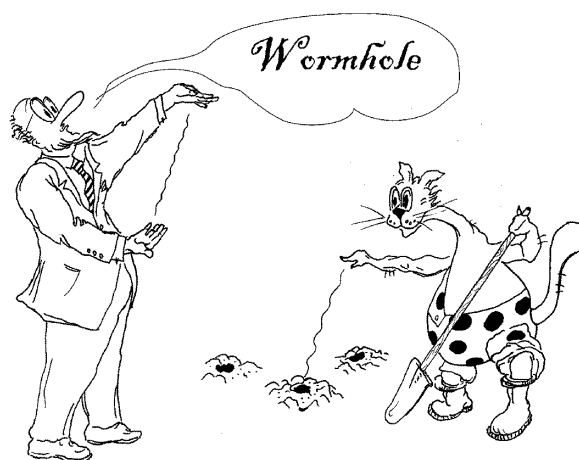
Figure 2. Wormhole.
