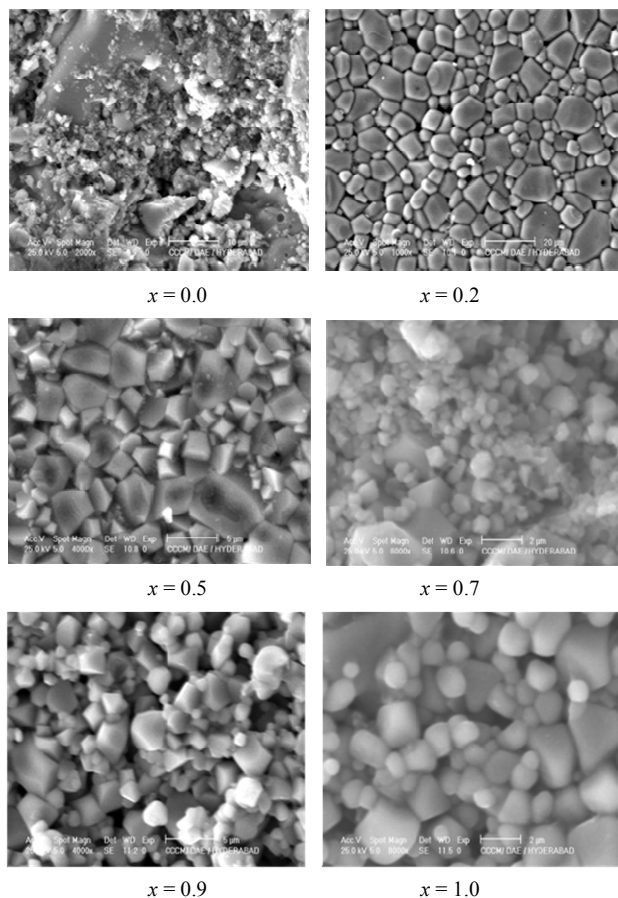
Figure 3. SEM images of \text{Ni}_{1-x}\text{Cu}_x\text{Fe}_2\text{O}_4 ( 0 \leq x \leq 1.0 ) ferrites.
