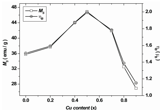
Figure 5. Variation of saturation magnetization and magnetic moment with Cu content x .
