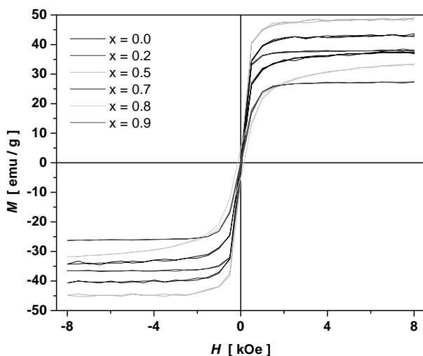
Figure 4. Hysteresis loops of \text{Ni}_{1-x}\text{Cu}_x\text{Fe}_2\text{O}_4 ( 0 \leq x \leq 1.0 ) ferrites.
