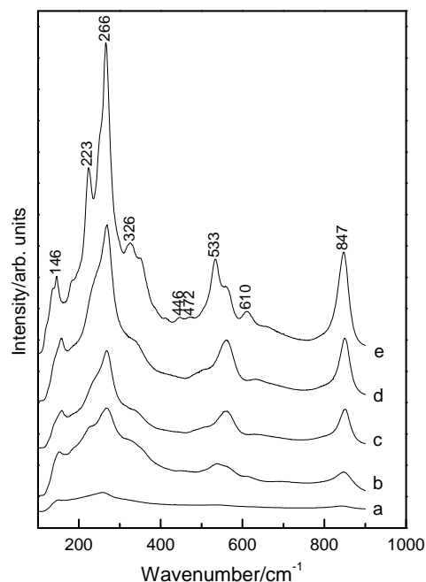
Figure 4. The evolution of the BTO Raman bands with temperature: (a) 90; (b) 450; (c) 550; (d) 650; and (e) 750°C
