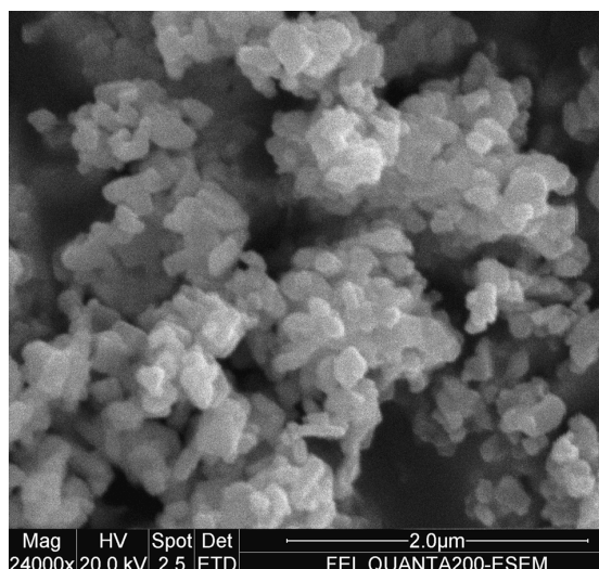
Figure 3. ESEM micrographs of nanocrystalline BTO calcined at 750°C for 5 min
