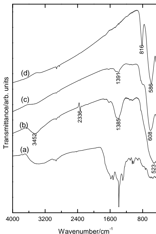
Figure 5. FTIR spectra of BTO precursor post-annealed at temperatures of 90 (a), 550 (b), 650 (c), and 750^\circ\text{C} (d) for 5\text{ min}
