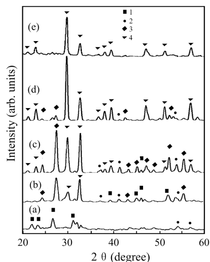
Figure 2. X-ray diffraction patterns of BTO precursor calcined at various temperatures of 90 (a), 450 (b), 550 (c), 650 (d), and 750°C (e). Peaks: (1) \text{Bi}_2\text{O}_3 , (2) \text{TiO}_2 , (3) \text{Bi}_{12}\text{TiO}_{20} , and (4) \text{Bi}_4\text{Ti}_3\text{O}_{12}
