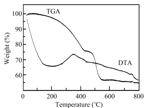
Figure 1. TG/DTA curves for stock precursors
