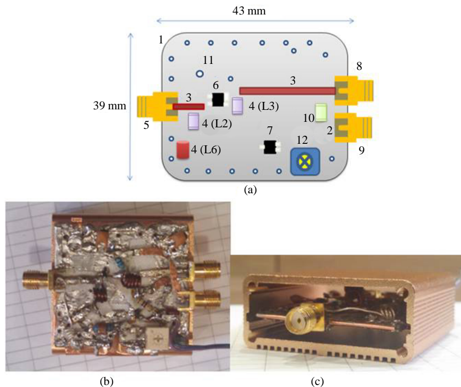
Figure 4. a) The suggested layout for the ULNA board. 1. FR4/PTFE Board, 2. Teflon Strip, 3. 50 Ω Micro-strip, 4. Inductors (this prototype used hand-wound inductors which were later replaced in following prototypes with HiQ SMD inductors), 5. SMA Connector, 6. HEMT transistor, 7. BJT transistor, 8. RF OUT, 9. DC OUT, 10. F/T LC Filter, 11. Via Holes, 12. Potentiometer, b) A photograph of our prototype; c) Cross sectional view of the unit while mounted in the case.
