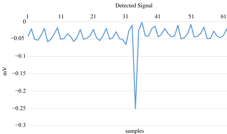
Figure 8. Detected resonant signal from a suspension of \text{CH}_3\text{OH} and \text{H}_2\text{O} with a 100 MHz source signal in a 1.48 \text{ T} \pm 0.1 \text{ T} magnetic field, as recorded with the DAQ in time-domain.
