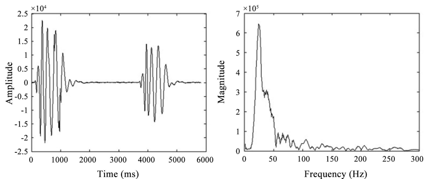
Figure 2. DFT calculation of an audio signal.
