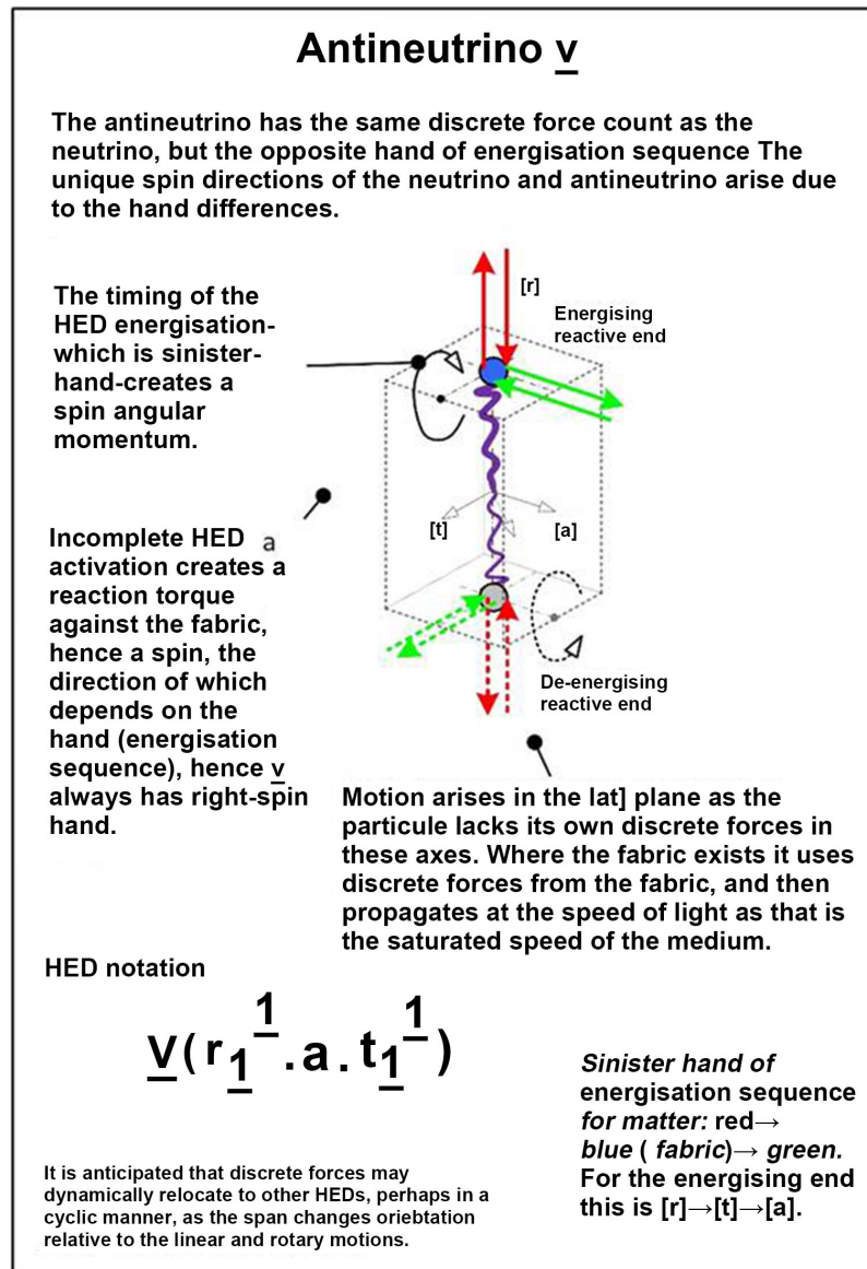
Figure 6. Proposed structure of the antineutrino, including internal structure and external discrete force structure. This particle spins in the opposite direction to the neutrino, because of the difference in energization sequence of the discrete forces. Image adapted with permission from [30].
