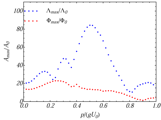
Figure 4. Particle momentum dependence of the ratio of averaged absolute value of the wave amplitude at a fixed final t > t_0 (when most of the energy of the system is concentrated in waves) to the initial amplitude at t = t_0 (when all energy of the system is concentrated in the YMC). The latter ratio accounts for the maximal deviation in the wave amplitudes within the time interval between t and t_0 . The results are shown for transverse \Phi and longitudinal \Lambda modes.
