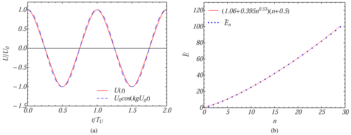
Figure 1. Numerical solution of the YM equation of motion (11) for the time dependence of free YMC potential, U = U(t) , and its analytical approximation (26) for a fixed initial phase \phi_0 = 0 (a) and numerical result for the energy spectrum of free YMC, E_n , and its continuous analytical approximation (29) (b).
