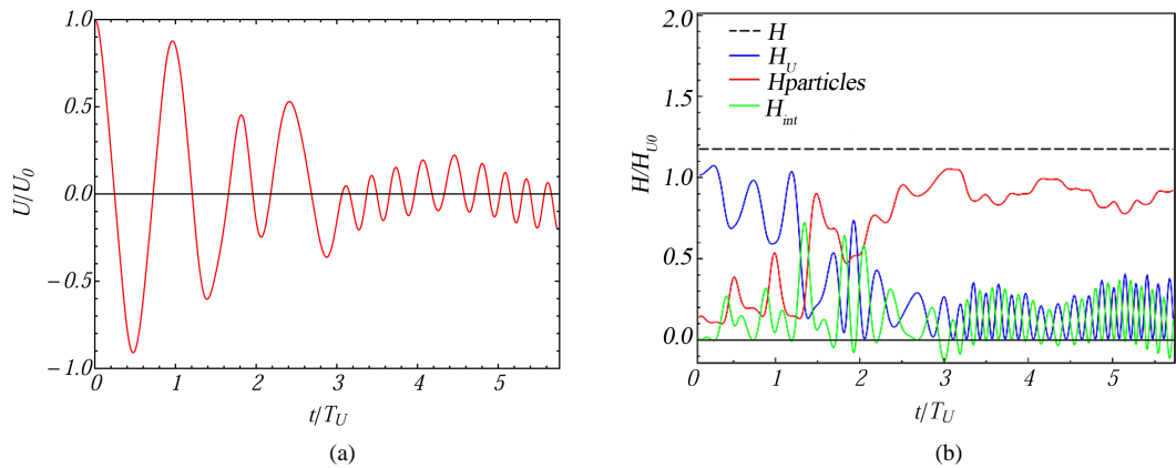
Figure 3. Time dependence of the YMC in the quasilinear approximation in the complete system of wave modes (a), and the evolution of condensate \mathcal{H}_U , YM wave modes (or particles) \mathcal{H}_{\text{particles}} , and interaction term \mathcal{H}_{\text{int}} contributions to the total energy in the complete system of wave modes (b). The illustrated numerical solutions are physical for relatively small wave amplitudes, i.e. \tilde{A}_k \ll U corresponding to t/T_U \lesssim 1 .
