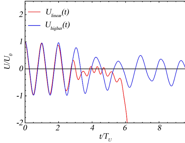
Figure 5. Time evolution of the YMC in the complete quasi-linear problem given by a numerical solution of Equations (16), (17) and (31) (red line) and in the problem with extra higher order terms included (36) (blue line).
