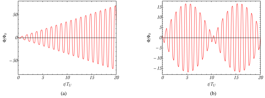
Figure 2. Example of normalized numerical solution of the system of YM Equations (11), (16) and (17) for one of the wave modes, \Phi = \Phi(t) , in the case of monotonic growth of oscillations for p=0 (a), and in the resonance-like instability domain with harmonic impulses for a particular value p=0.1gU_0 (b).
