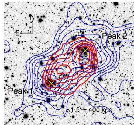
Figure 20. The A1758N merger from B. Ragozzine et al. [63]. The blue contours represent the weak lensing mass reconstruction made from a background galaxy density of 24.0 galaxies/arcmin 2 . The outer blue contour begins at surface mass density \kappa = 0.07 and each contour increases in steps of 0.045 up to \kappa = 0.34 . The red contours follow the X-ray gas mass obtained in the Chandra exposure. The NW cluster's BCG aligns with the X-ray gas and the weak lensing peak. The SE cluster's BCG and weak lensing peak are well separated from the X-ray gas, which has a bright peak near the midpoint of the two weak lensing peaks.
