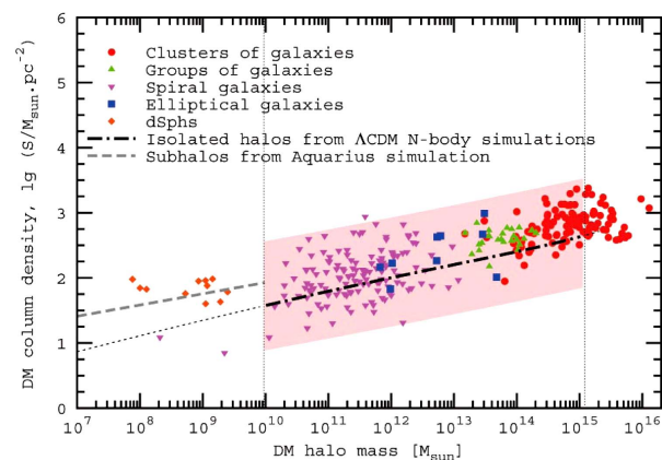
Figure 11. Dark matter column density vs. dark matter halo mass in solar units. From A. Boyarsky et al. [47].
