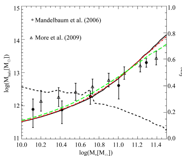
Figure 10. Dark matter halo mass M_{halo} as a function of stellar mass M_* . The thick black curve is the prediction from abundance matching assuming no dispersion in the relation between the two masses. Red and green dashed curves assume some dispersion in \log M_* . The dashed black curve is the satellite fraction as a function of stellar mass, as labeled on the axis at the right-hand side of the plot. From Qi Guo et al. [46].
