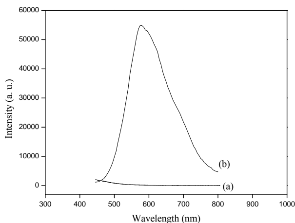
Figure 3. PL spectra ( \lambda_{ex} = 360 nm) of: (a) Pure KCl and (b) KCl doped AuCl nanocrystals.
