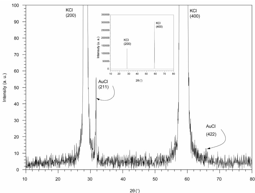
Figure 2. X-ray spectrum of KCl single crystals doped AuCl after annealing at 650°C for 3 h.
