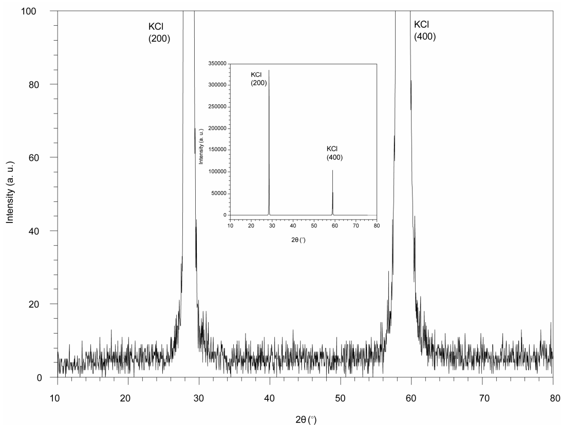
Figure 1. X-ray spectrum of pure KCl single crystals.
