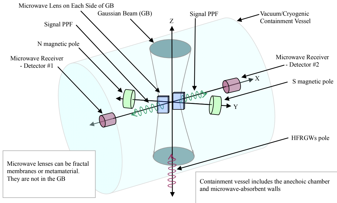
Figure 7. Schematic of the Li-Baker HFRGW detector, exhibiting microwave lenses on each side of the GB focusing PPF on the microwave receivers.
