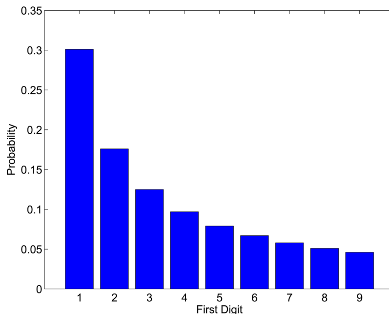
Figure 1. Probability distribution of Benford's law.
