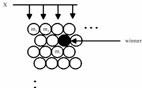
Figure 5. Self-organizing map
