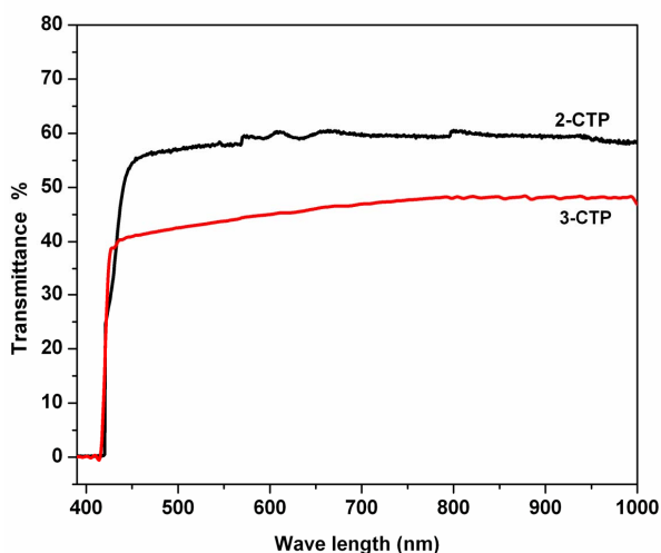
Figure 8. Vis-IR spectra of 2-CTP and 3-CTP single crystals.
