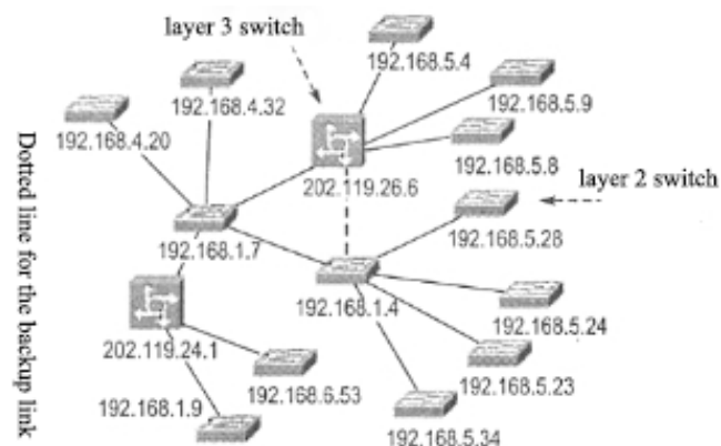
Figure 2. Part of data-link level's topology.
