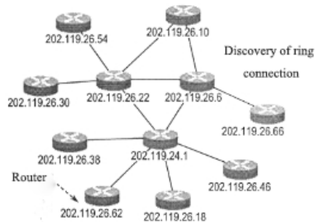
Figure 1. Topology of network level.
