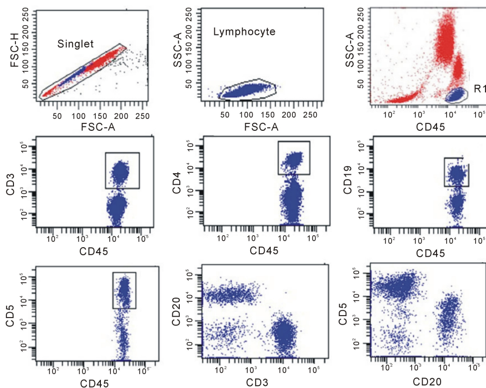
Figure S2. Gating Strategy for percentage of positive cell subset typing. A doublet exclusion gate based upon (FSC-A vs. FSC-H) was utilized to gate on singlet cells (upper left dot plot), and within this singlet cell gate, a lymphocyte gate was drawn in a dot plot of FSC-A vs. SSC-A (Upper middle dot plot). Using a dot plot of CD45 vs. SSC-A under the lymphocyte gate, R1 gate was drawn around the CD45 positive cells and used for all subsequent gating (dot plots of CD45 vs. CD3, CD45 vs. CD4, CD45 vs. CD19, CD45 vs. CD5, CD3 vs. CD20 and CD20 vs. CD5 were shown).
