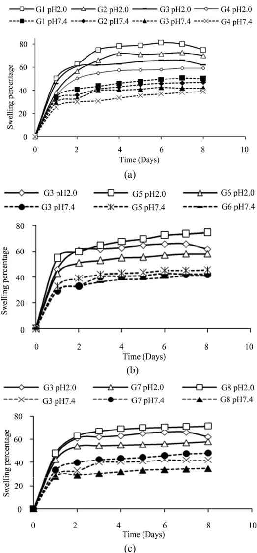
Figure 1. (a) Swelling behavior of crosslinked beads as a function of time in solution pH 2.0 and pH 7.4 at 37°C having different percentage of glutaraldehyde; (b) Swelling behavior of crosslinked beads as a function of time in solution pH 2.0 and pH 7.4 at 37°C having different weight ratio of chitosan; (c) Swelling behavior of crosslinked beads as a function of time in solution pH 2.0 and pH 7.4 at 37°C having different weight ratio of amino acids.
