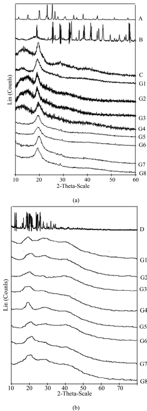
Figure 4. (a) X-ray Diffraction (XRD) graphs of glutamic acid (A), glycine (B), chitosan powder (C) and drug unloaded crosslinked beads (G1-G8); (b) X-ray Diffraction (XRD) graphs of pure chlorpheniramine maleate (CPM) drug (D) and drug loaded crosslinked beads (G1-G8).
