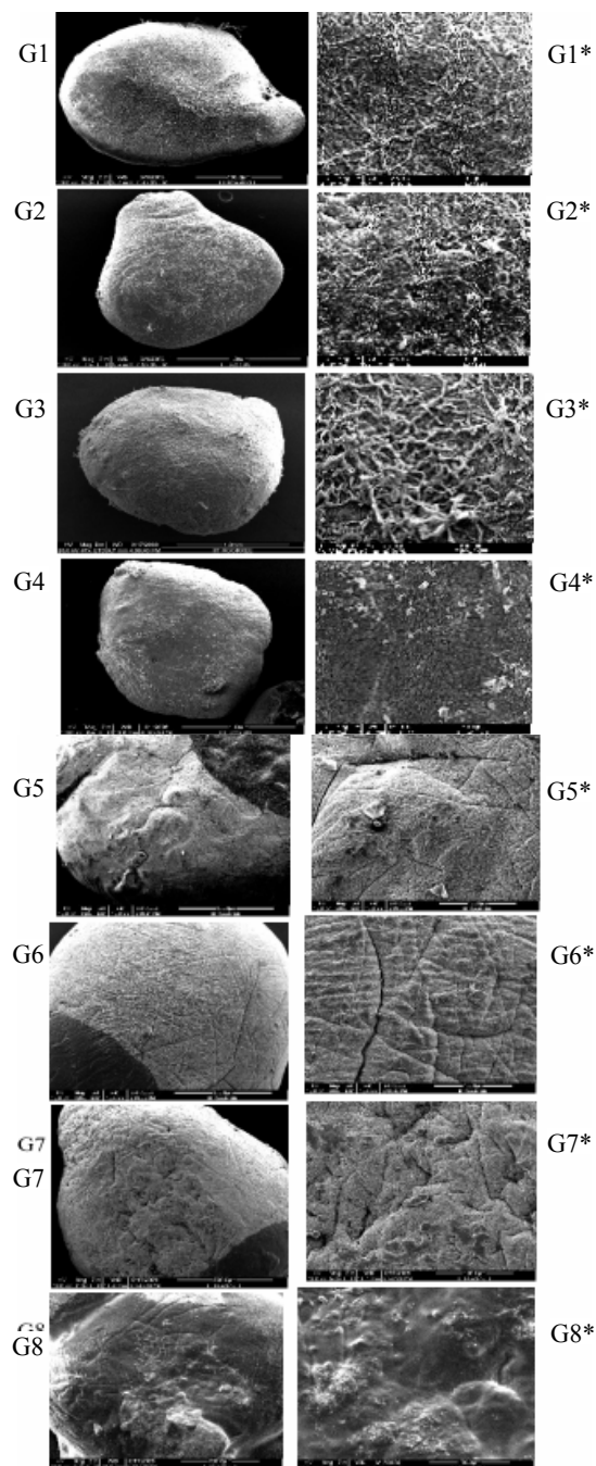
Figure 2. Scanning Electron Microscopy (SEM) photographs of crosslinked beads (G1-G8) and their magnified photographs showing surface morphology (G1*-G8*).
