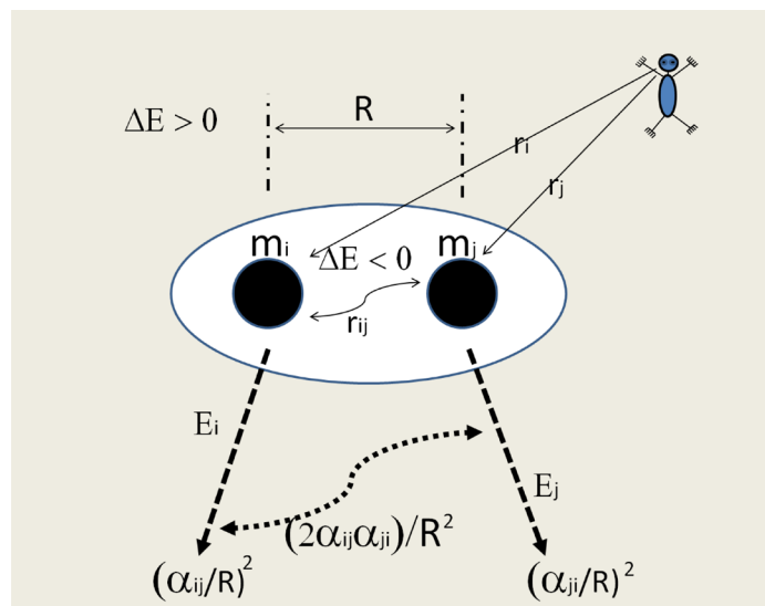
Figure 3. Energy transfer from the pair to the surroundings and the sub-space (white area) with internal exchanges as observed from far away.
