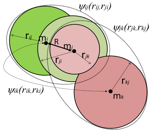
Figure 2. Forming and describing of \mathcal{N} = N!/2(N-2)! Pairs. In this example the number of groups is three.
