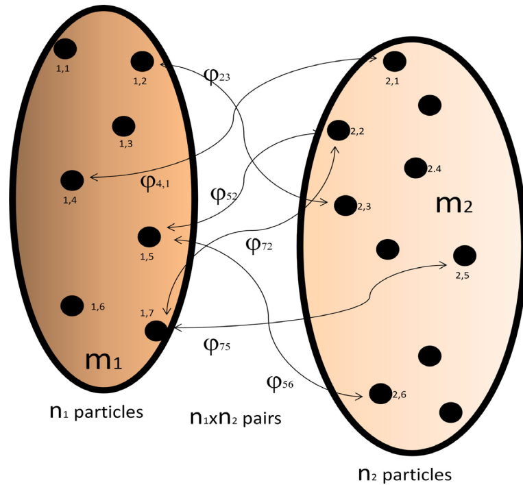
Figure 4. Interaction between masses by building up structures from equal mass units.
