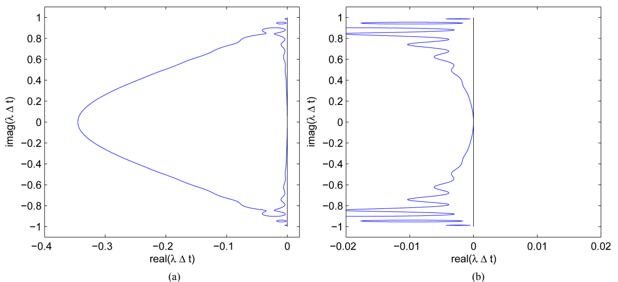
Figure 4. (a): Absolute stability region of method M2. (b): close up of the stability region along the imaginary axis.
