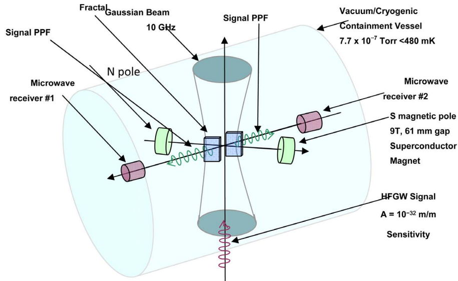
Figure 10. Notional drawing of Li-Baker detector by the author.
