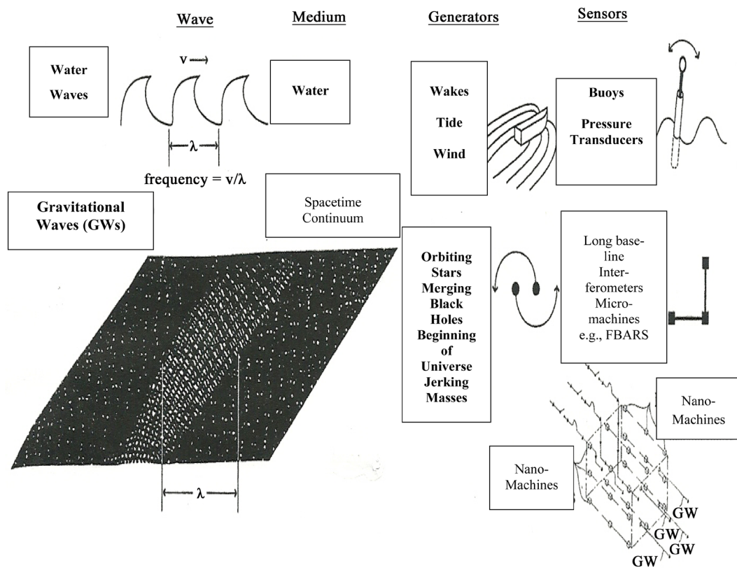
Figure 5. Gravitational waves.
