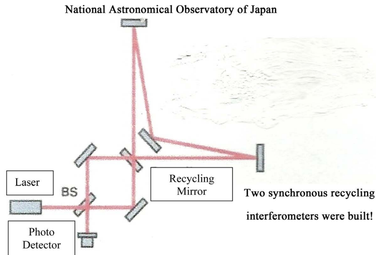
Figure 8. National astronomical observatory of Japan 100 MHz HFGW detector (Nishizawa, et al. , [70]).
