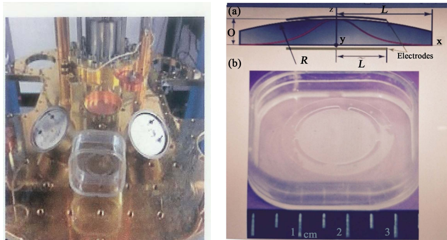
Figure 11. Gravitational wave detection with high frequency phonon trapping acoustic cavities (Goryachev and Tobar [81]).
