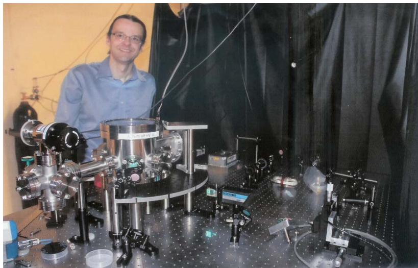
Figure 9. Stanford/university of Nevada HFGW detector 50 to 300 kHz [4].
