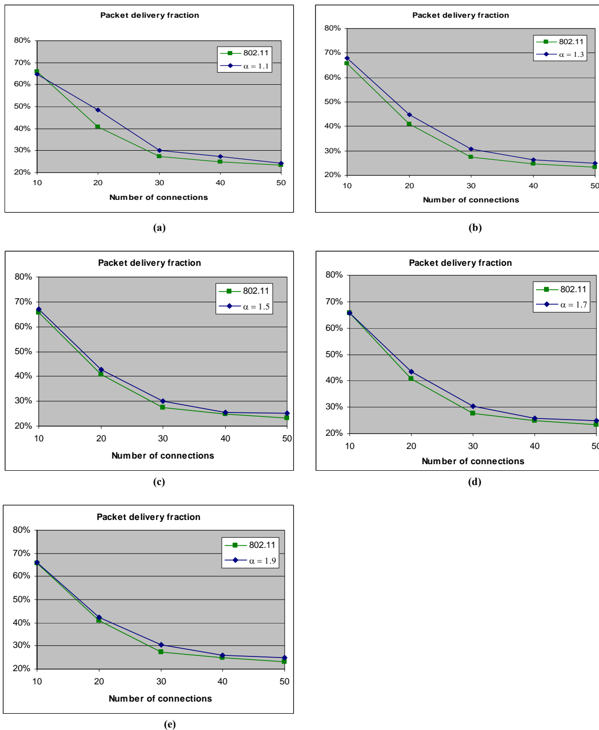
Figure 1. PDF of HBAB ( \alpha = 1.1, 1.3, 1.5, 1.7 and 1.9 ) vs BEB-simulation.
