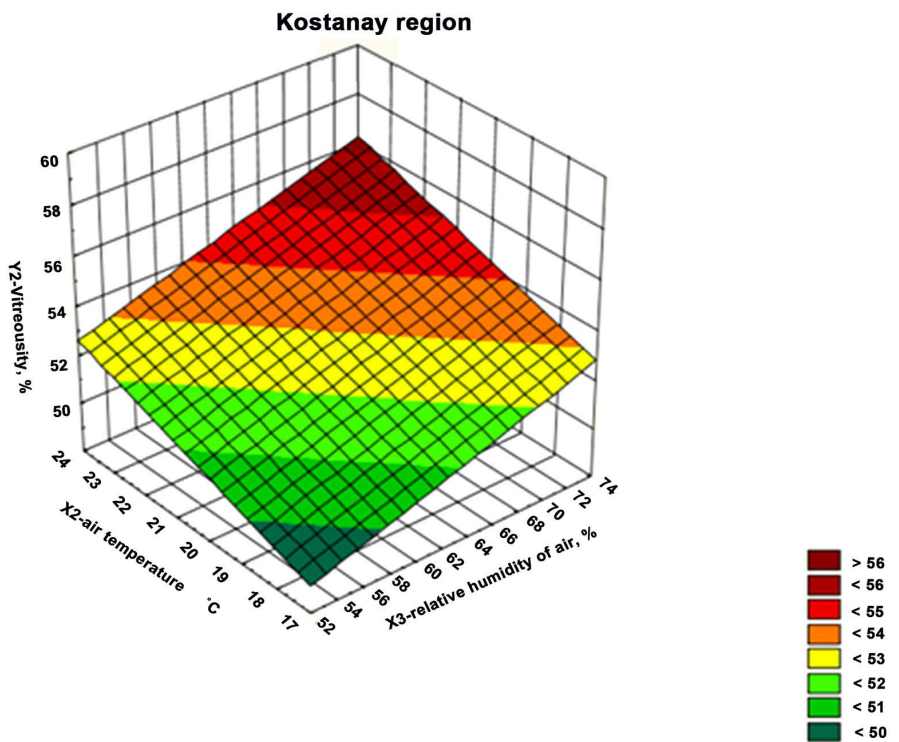
Figure 2. Y_2 —Vitreosity, % = 31.9146 + 0.1678 \cdot X_3 + 0.4985 \cdot X_2 .
