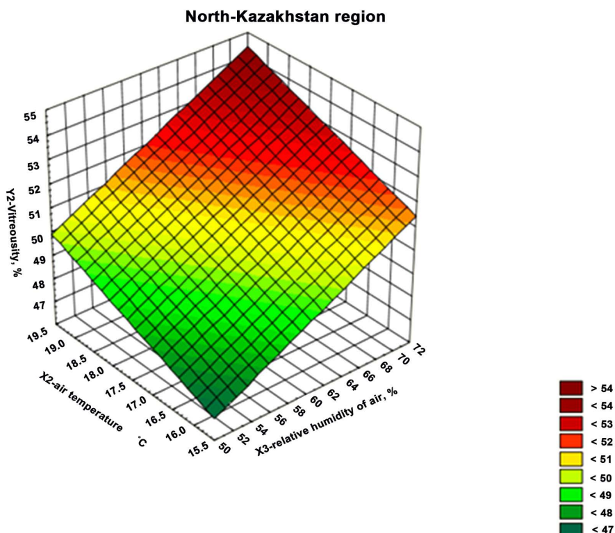
Figure 3. Y_2 —Vitreosity, % = 25.0994 + 0.2041*x + 0.7486*y.
