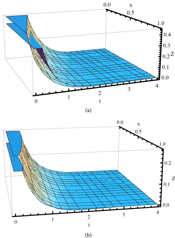
Figure 3. (a) w_x(x,t) - w_t(x,t) and p_5(x,t) ; (b) w(x,t) and p_9(x,t) .
