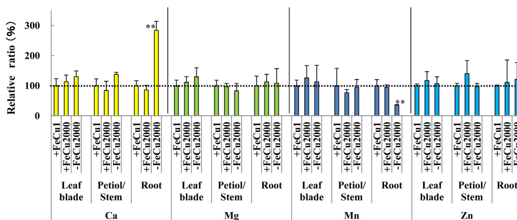
Figure 4. Minerals (Ca, Mg, Mn and Zn) contents in the various organs. Seedlings were subjected to different Cu/Fe concentrations and cultured under long day (LD) conditions for 4 weeks. +Fe, with 100 \mu M Fe(III)-EDTA; -Fe, without Fe; Cu1, 0.1 \mu M CuSO 4 ; Cu2000, 200 \mu M CuSO 4 . Control (+FeCu1) is expressed as 100%. Others are expressed as relative values. Data are means and sd of 4 samples. Data are analyzed by ANOVA and Student t -test. **Reveals significant differences at the levels of P < 0.01 compared with control.
