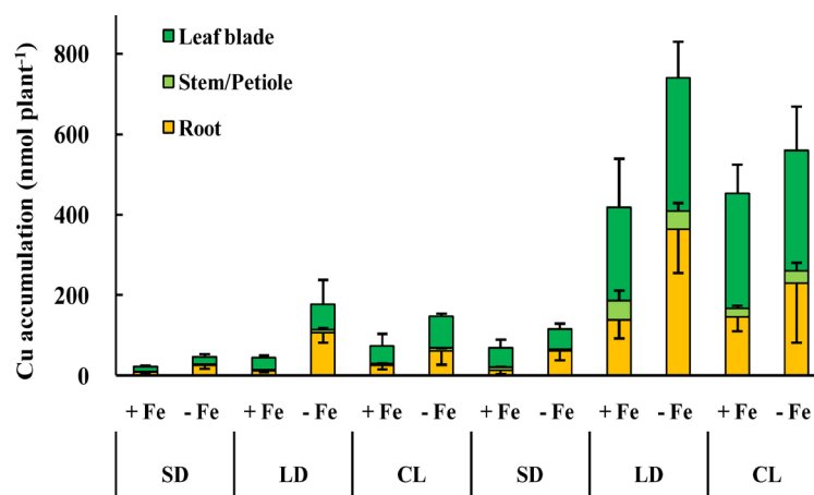
Figure 2. Cu distribution in various organs of H. albus plants. Seedlings were treated with Cu excess (200 \mu\text{M} ) in combination with/without Fe for 2 and 4 weeks at 25°C on a rotary shaker at 50 rpm in the incubator, under three different light regimes (121 \mu\text{mol}\cdot\text{m}^{-2}\cdot\text{s}^{-1} ): short day (SD), 10 h light - 14 h dark; long day (LD), 16 h light - 8 h dark; continuous light (CL), 24 h light. -Fe, no addition of Fe; +Fe, with addition of 100 \mu\text{M} Fe(III)-EDTA. Data are means and sd of 4 samples.
