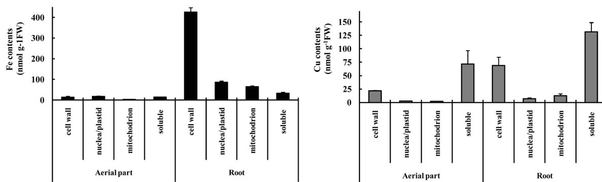
Figure 3. Cu and Fe allocations in various fractions from aerial parts and roots. Seedlings supplied with Cu excess (200 \mu\text{M} ) together with Fe (100 \mu\text{M} ) were cultured under long day (LD) condition for 4 weeks. Freshly harvested tissues ( ca. 2 g) were ground in 50 mM Tris-HCl buffer (pH 7.5) containing 250 mM sucrose and 10 mM DTT at 4°C and then filtered through nylon mesh (84 mm) in vacuo . Cell wall was recovered on the filter. The filtrate was centrifuged at 880 \times g, followed by 21,880 \times g; the pellets were denoted as “nucleus and plastids fraction” and “mitochondrial fraction”, respectively, and the rest of the solute as “soluble fraction”. Experiments were repeated three times and the average and standard deviation are given.
