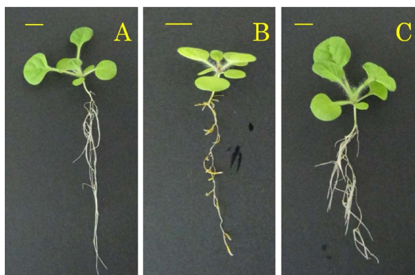
Figure 1. H. albus seedlings treated with three different Cu/Fe concentrations. Seedlings were incubated for 2 weeks at 25°C on a rotary shaker at 50 rpm in the incubator under long day (LD) conditions, 16 h light ( 121 \mu\text{mol}\cdot\text{m}^{-2}\cdot\text{s}^{-1} ) - 8 h dark. Photos: (A) A control plant treated with \text{CuSO}_4 (0.1 \mu\text{M} ) and Fe(III)-EDTA (100 \mu\text{M} ) in B5 basal medium; (B) A plant subjected to Fe deficiency by treatment with B5 Cu (0.1 \mu\text{M} ) without Fe (-Fe); (C) A plant subjected to Cu excess (200 \mu\text{M} ) in combination with Fe deficiency (-Fe). Bars indicate 1 cm.
