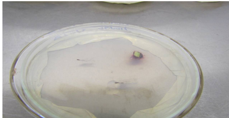
Plate 3. Four days old callus (Phase II).
