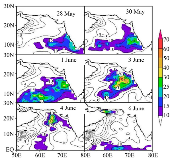
Figure 6. Sensible heat flux in the Arabian Sea for various intensities of the cyclone, Gonu during 28 May to 6 June.
