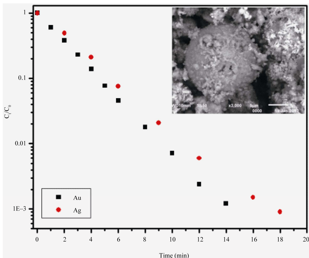
Figure 3. First-order plots showing removal of gold and silver from cyanide solution.
