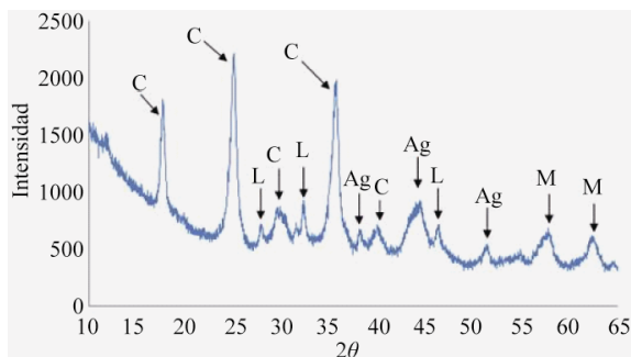
Figure 5. X-ray diffractogram of solids obtained in the recovery of gold and silver C: Cu_2Fe(CN)_6 \cdot 2H_2O , A: Silver, M: Magnetite and L: Lepidocrocite.
