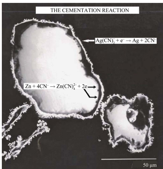
Figure 1. Electrochemical reaction of cementation of silver on zinc particle.
