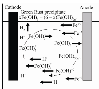
Figure 2. An illustration of the EC mechanism (arrow indicate the migration of ions, the H_2 evolution and the formation of green rust).
