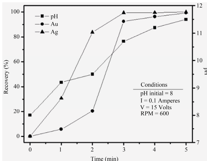
Figure 4. Gold and silver recoveries from Bacis cyanide solutions and pH vs EC residence time.
